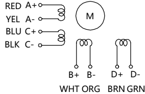
Wiring Diagram
