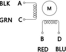
Wiring Diagram
