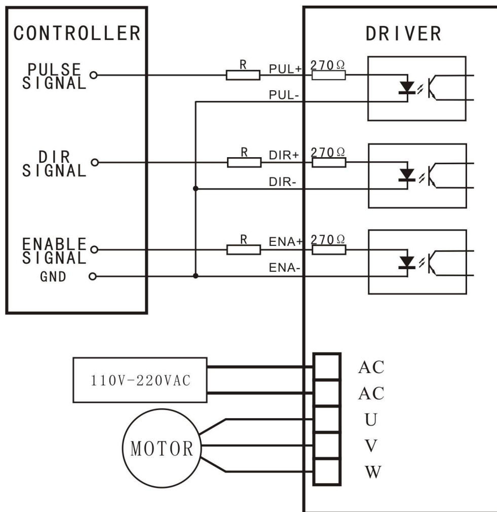
Figure 3: Typical connection
